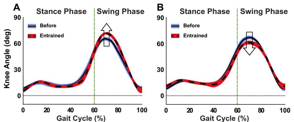
Fig. A1. Knee angle trajectory (mean \pm SD) across the gait cycle (in percent) for a selected subject during TM-longer (A) and TM-shorter (B) trials. In both conditions, the mean knee excursion and SDs are depicted for the 15 consecutive strides before perturbations (solid line) and the last 15 strides during perturbation (dashed line). During TM walking, peak knee flexion increased (upward arrow) upon entrainment to longer \tau_p via an increase in stride length. Conversely, peak knee flexion decreased (downward arrow) upon entrainment to shorter \tau_p via a decrease in stride length, given the constant treadmill belt speed.
